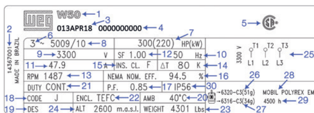
Figure 26 - Main nameplate of the motor.
